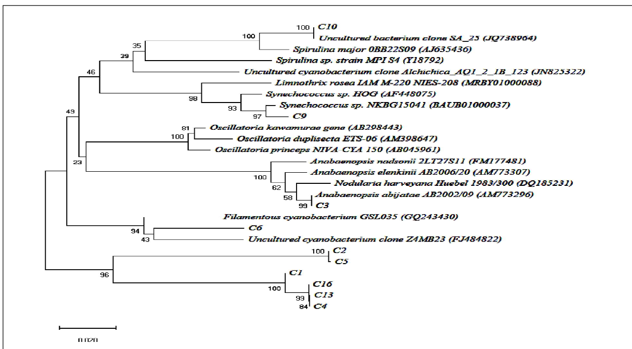
Figure 4: Unrooted phylogenetic tree showing the relatedness of the cultured cyanobacterial isolates to closest relatives
