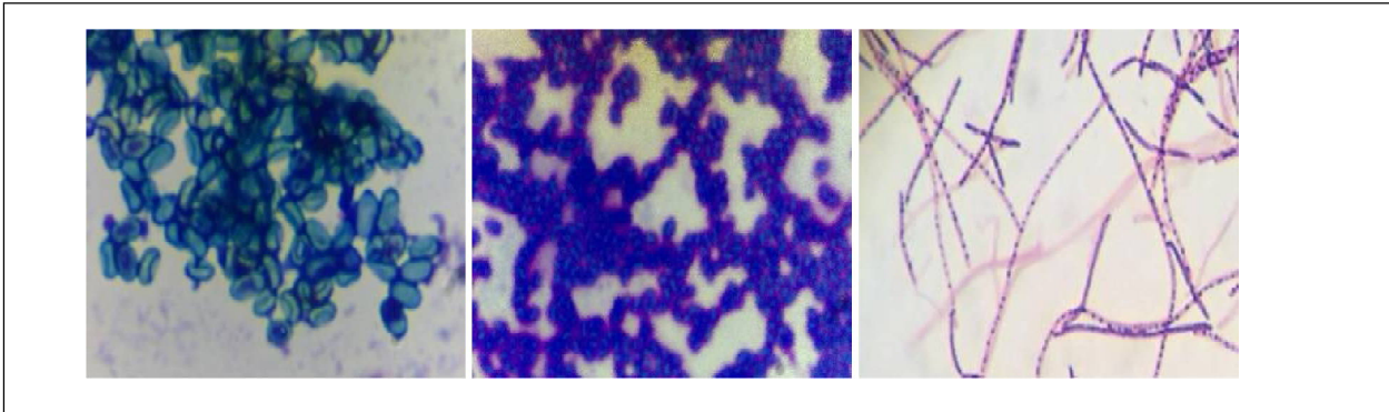
Figure 3b: Microscopic images of the isolates C13, C14, C16 grown on solid medium as seen under a compound microscope at x400
