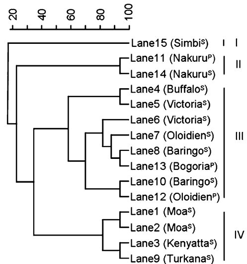
Fig. 3. A dendrogram generated by cluster analysis (UPGMA – Pearson's correlation index) showing the relationship of DGGE fingerprinting of 16S rRNA genes obtained from sediment and planktonic samples from Kenyan lakes. S, sediment samples; P, planktonic samples.
