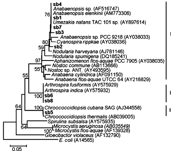
Fig. 4. NJ tree based on partial 16S rRNA gene sequences showing the phylogenetic relationship among sequences from excised bands from DGGE of sediment and planktonic samples from Kenyan lakes (bold), with reference sequences obtained through BLAST analysis. Bootstrap values > 50 were included.
