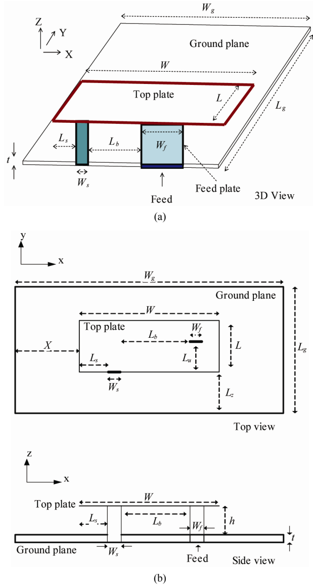
Figure 1. (a) Planar inverted-F antenna under study; (b) Geo-metry of PIFA structure.
